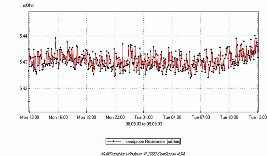
Figure 5-2: Metal loss plot on sand probe
