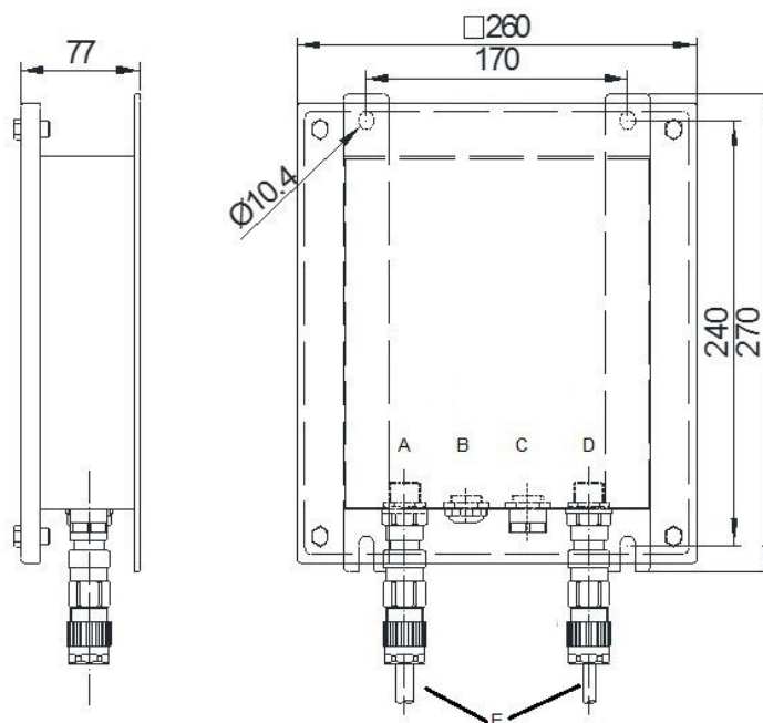
Figure 4-1: Footprint of CorrLog and SandLog
